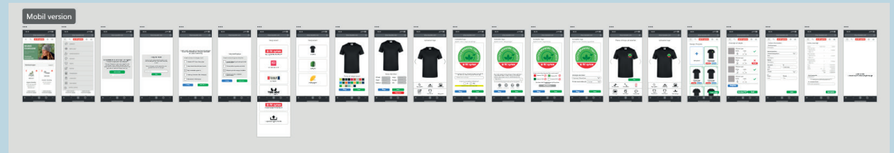
Mobil flow
